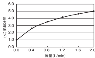
形D6F-02A1-110
