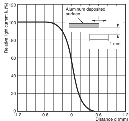
Fig 9. Sensing Position Characteristics (Typical)
